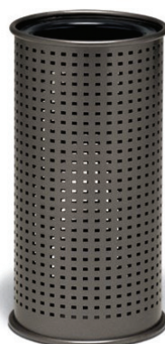
AEG531C ▲ W: 12 3/8" D: 12 3/4" H: 23 3/8-24 1/8"* * varies with material options
